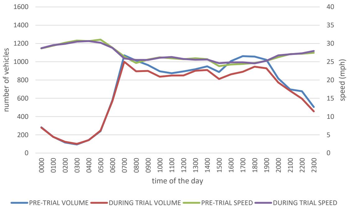
Speed/volume before and during trial - CROUCH END HILL
