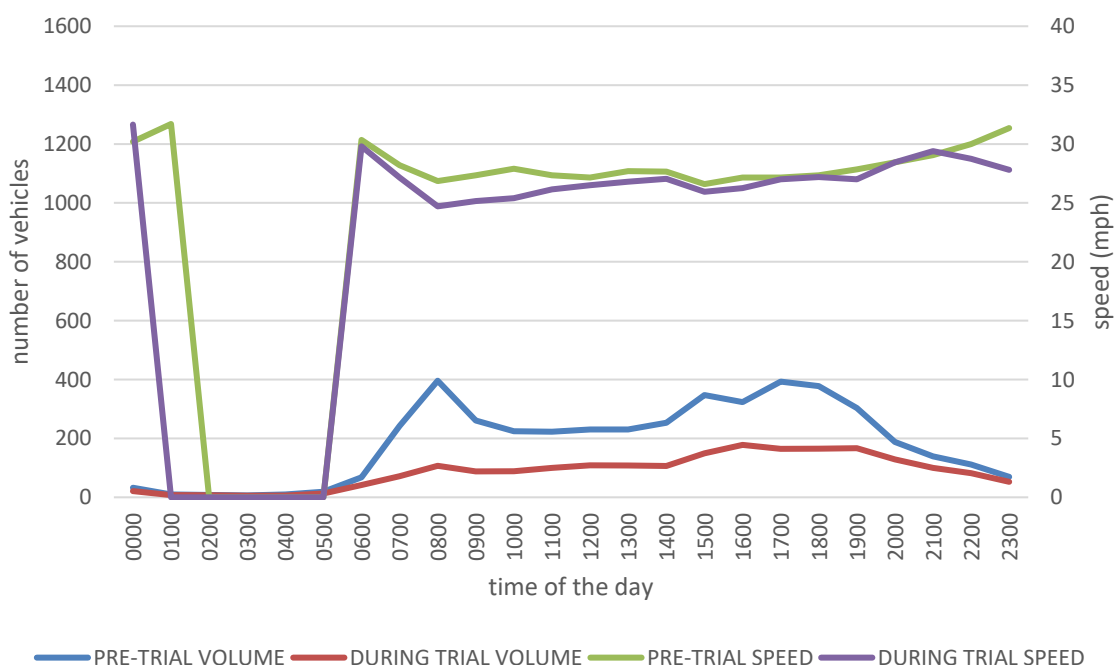
Speed/volume before and during trial - ROKESLY AVENUE
