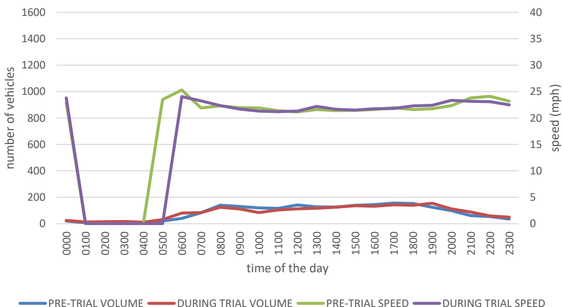
Speed/volume before and during trial - ELDER AVENUE (north of Tottenham Lane)
