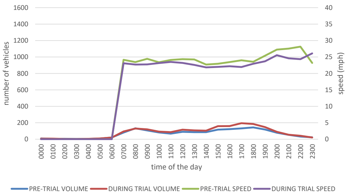
Speed/volume before and during trial - CHRISTCHURCH ROAD
