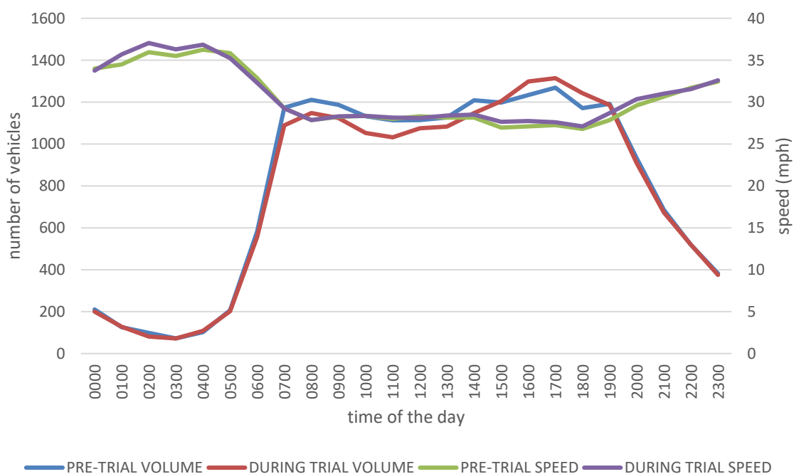
Speed/volume before and during trial - PRIORY ROAD
