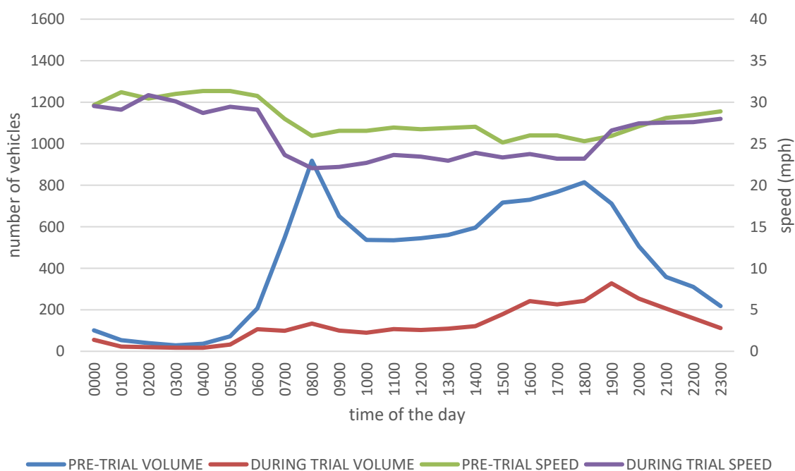
Speed/volume before and during trial - MIDDLE LANE
